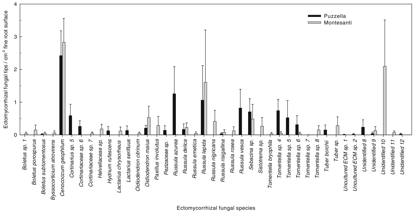
Fig. 3 Mean specific tip density for each ectomycorrhizal fungal species±SE from Puzzella a healthy Castanea sativa stand and Montesanti a Castanea sativa stand with Phytophthora infected trees
