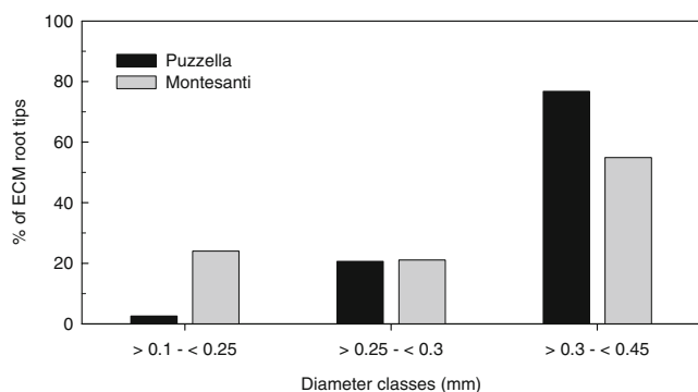
Fig. 4 The number of ECM root tips divided into three root diameter classes of root tip initials expressed as a percentage of the total number of ECM tips sampled at the Puzzella and Montesanti stands
