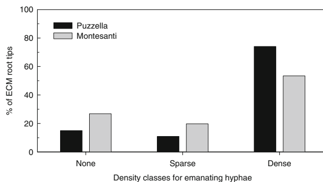
Fig. 5 The number of ECM root tips divided into three hyphal density classes expressed as a percentage of the total number of ECM tips sampled at the Puzzella and Montesanti stands
